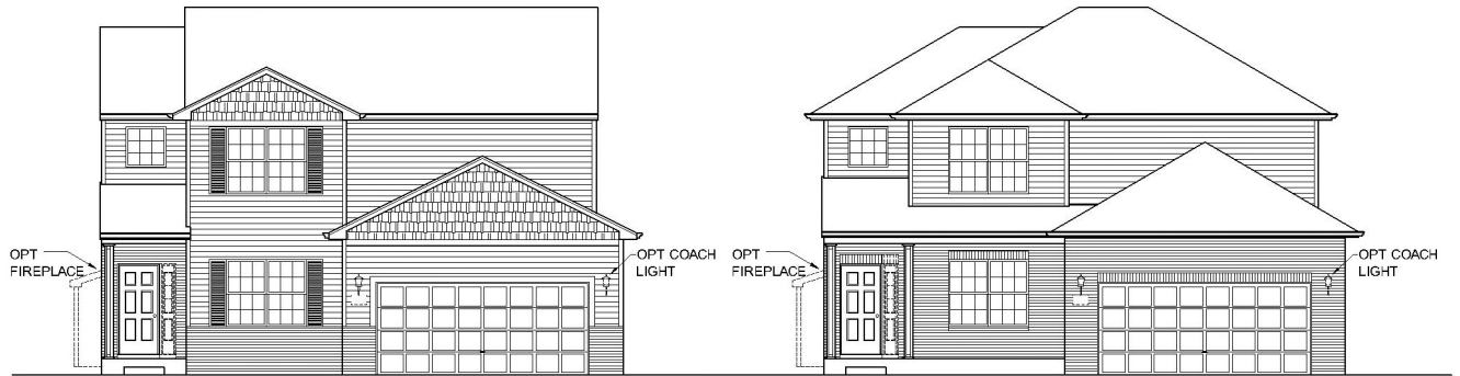
HORIZONTAL SIDING, BRICK, SHAKES FRONT ELEVATION "B"
