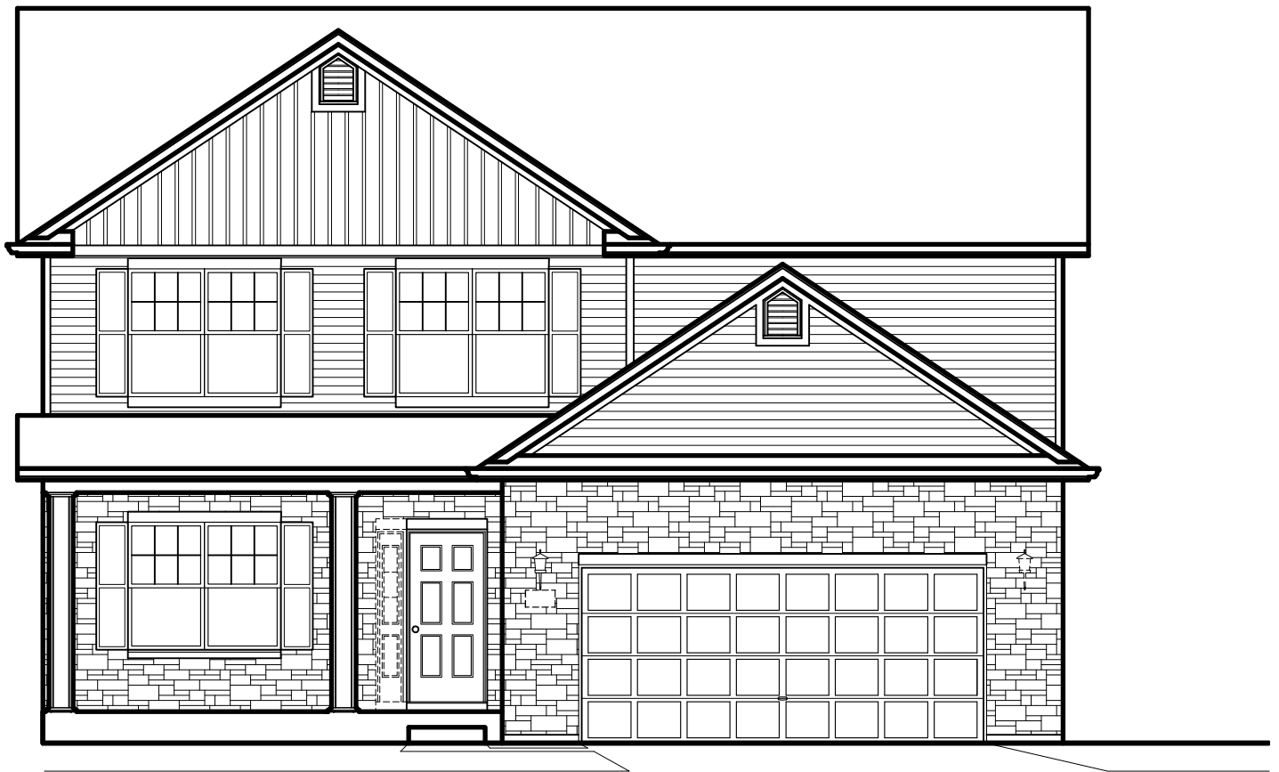
ELEVATION "D"
