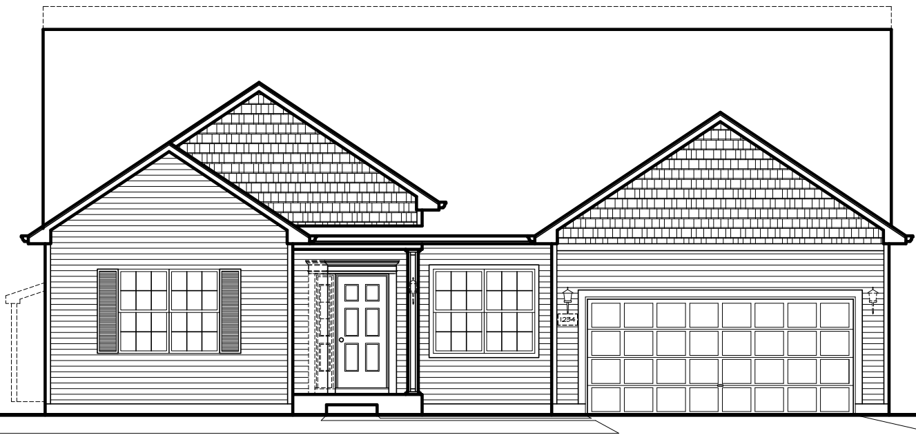
ELEVATION "A"
