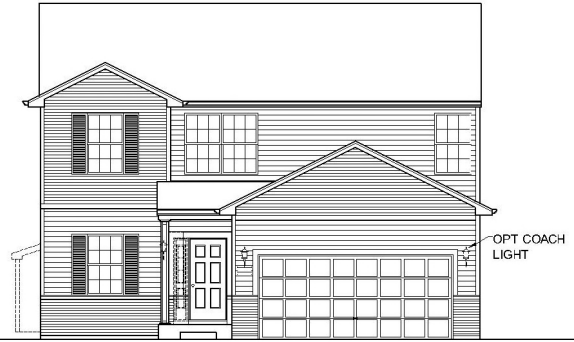
4" HORIZONTAL SIDING, 3" HORIZONTAL ACCENT SIDING, BRICK WAINSCOT FRONT ELEVATION "1"
