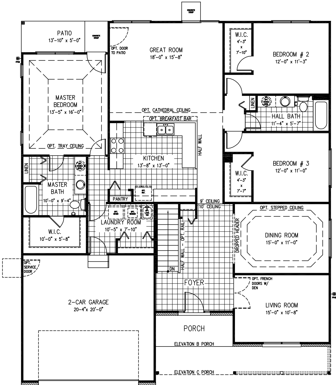
FIRST FLOOR PLAN – 9'-0" CEILING (UNLESS NOTED OTHERWISE) MANCHESTER – 2124 SQ. FT.
