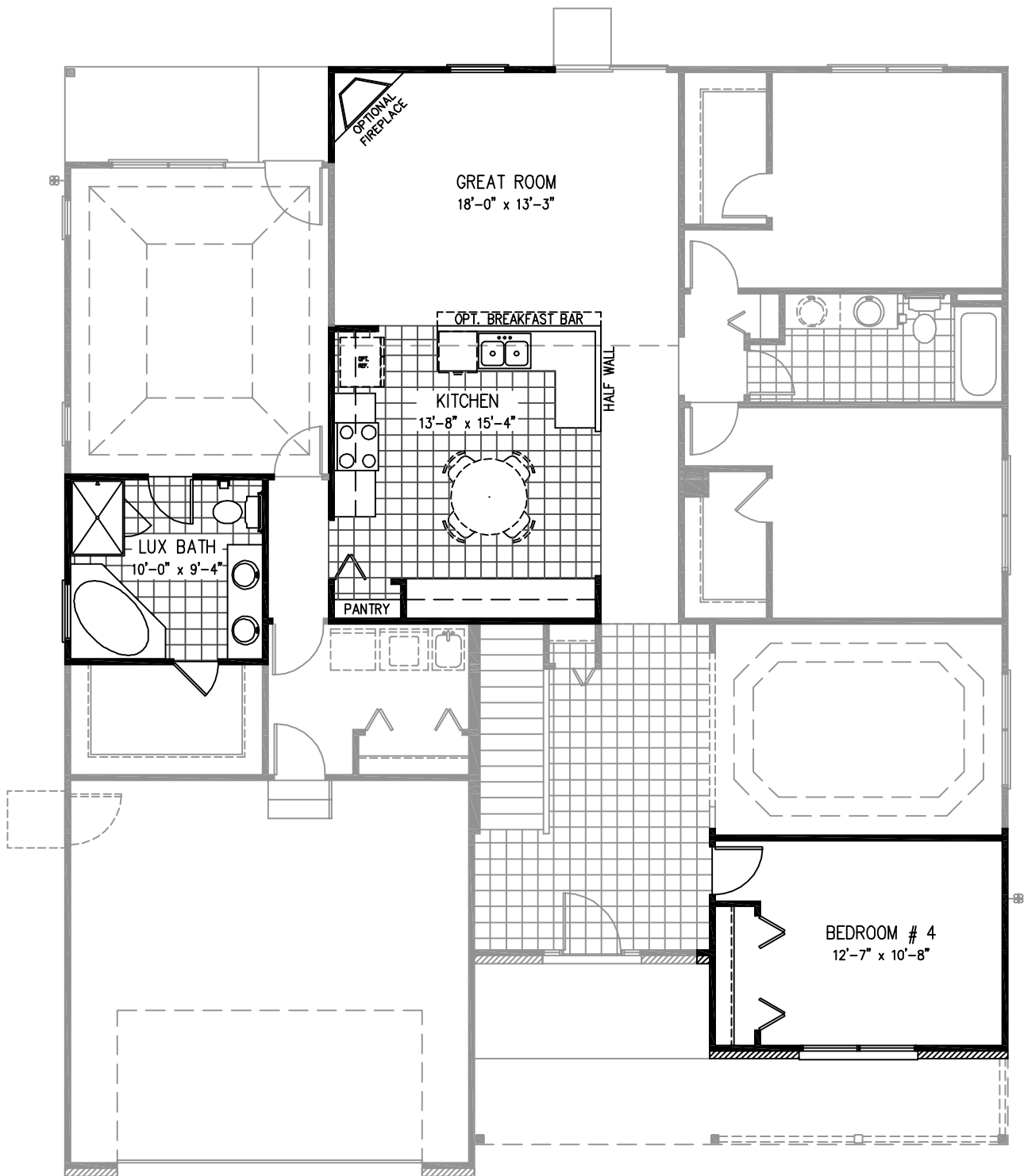
FIRST FLOOR PLAN OPTIONS (9'-0" CEILING UNLESS NOTED OTHERWISE) MANCHESTER — 2124 SQ. FT.
